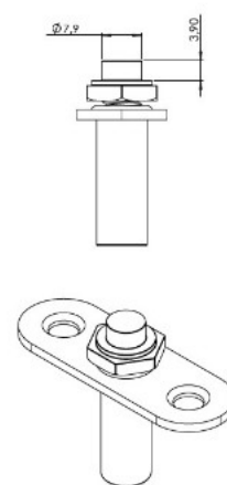
BOTTOM FITTING
