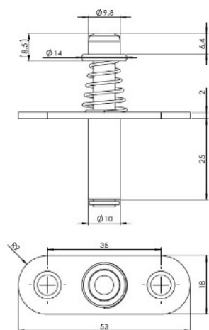
TOP FITTING
